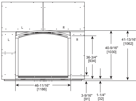
Arched Firescreen
