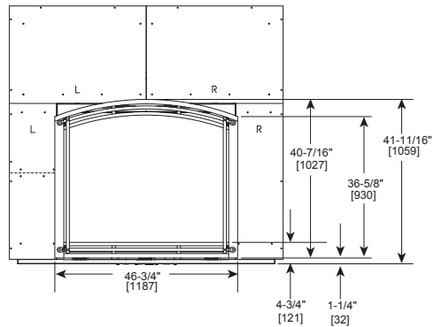
Arched Forge
