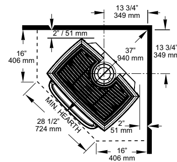
Figure 95. Corner installation clearances and minimum hearth pad.
