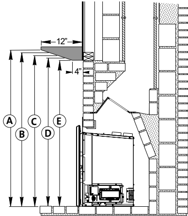
Figure 123. Mantel and ceiling clearances
