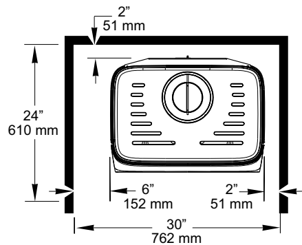
Figure 51. Alcove Clearances.
