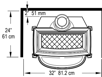
Figure 64. Alcove Installation Clearances.
