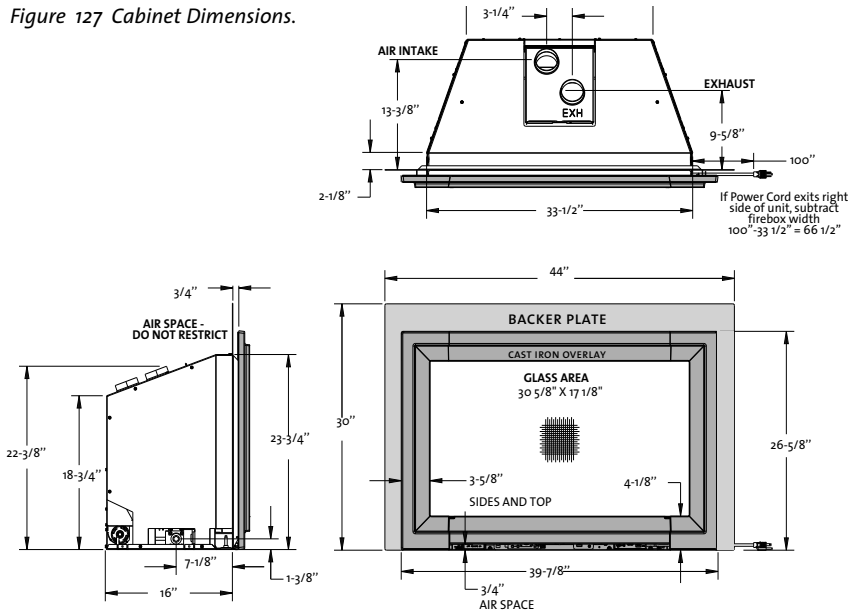
Figure 127 Cabinet Dimensions.
