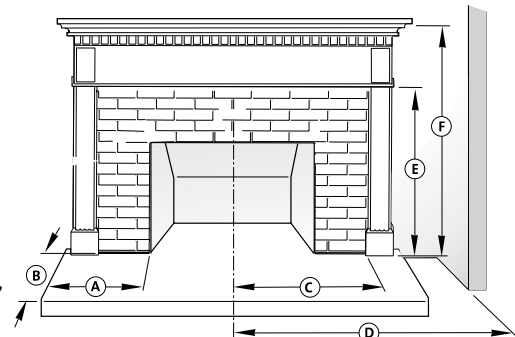
Figure 106. Clearance requirements
