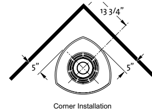
Figure 57. Corner installation Top Exit vent adaptor centerline at minimum clearance.
