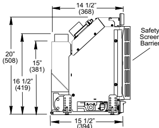
Figure 102. GI 450 DV Katahdin dimensions.
