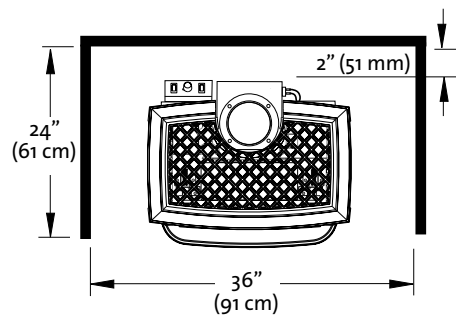
Figure 133 Alcove Installation Clearances.
