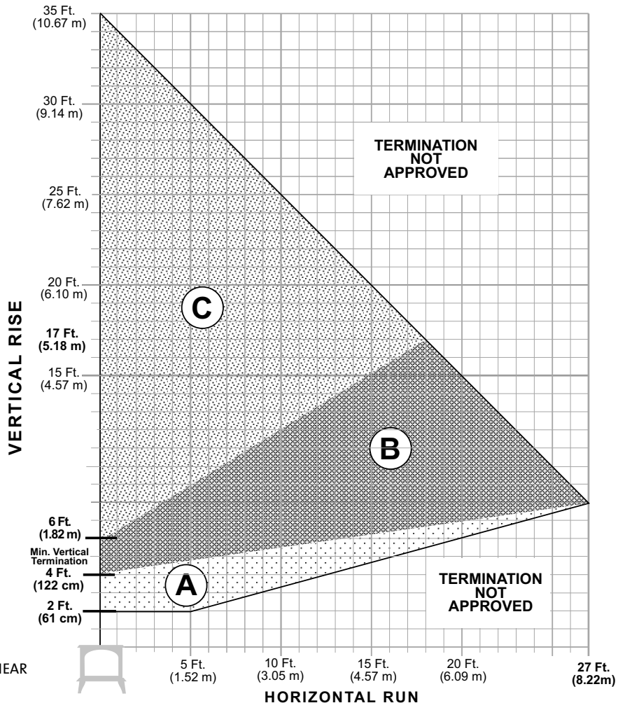
Figure 91. Vent Termination Zone Matrix - NG / LP
